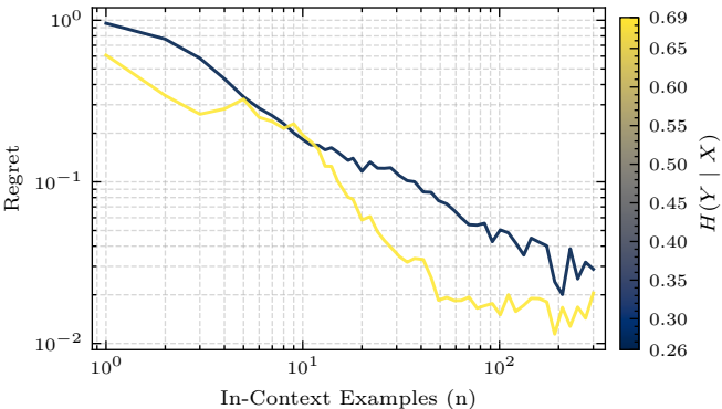
In-Context Learning Regret for Qwen-2.5 (7B)
